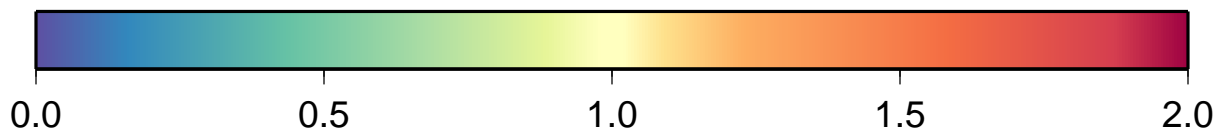
UCERF3/UCERF2 Time Dep Ratio
