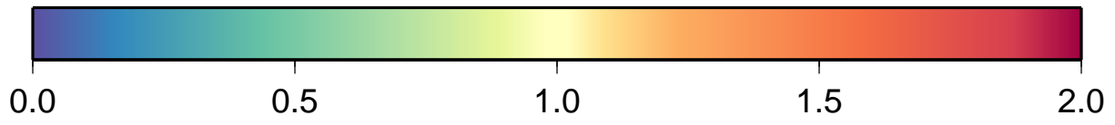
UCERF3 Mean BPT/Poisson Prob Gain
